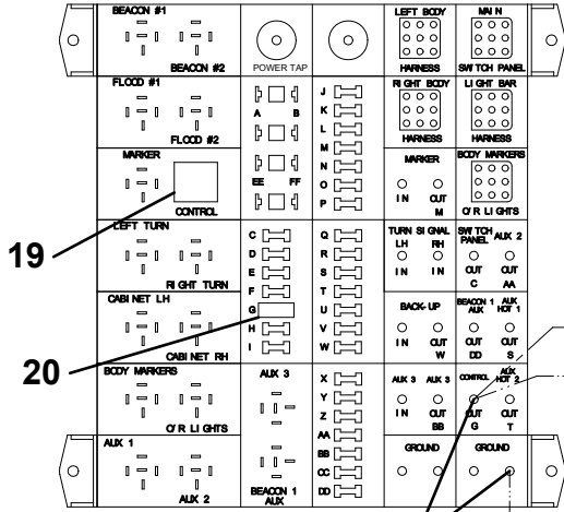
POWER PANEL, REF
