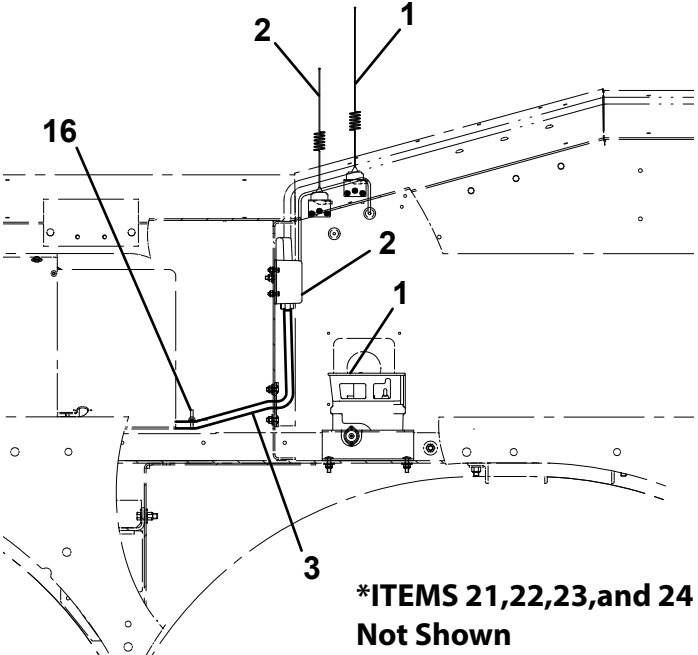
POWER PANEL, REF
