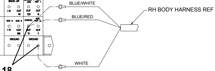
POWER PANEL, REF
